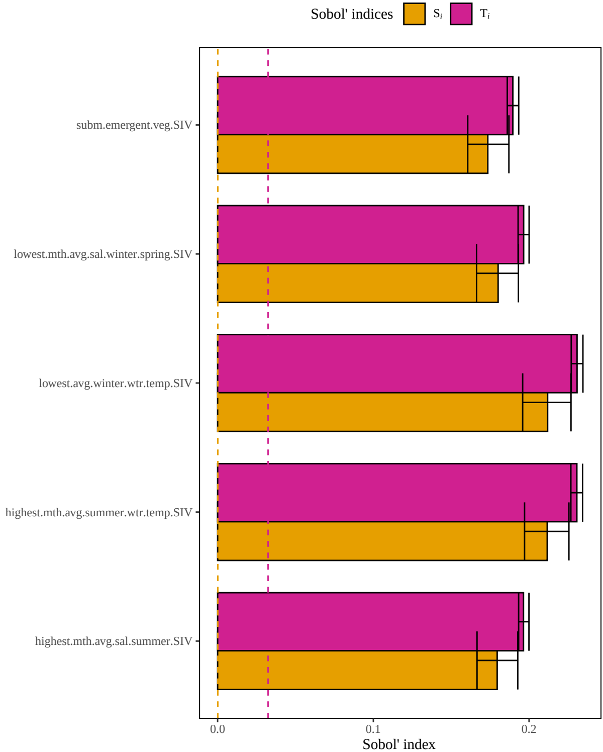
Figure 5. Results of a sensitivity analysis for the spottedseatrout model based on a geometric mean structure. Dashed lines represent baseline numerical approximation error for S_i and T_i ( i.e. , dummy variables).
